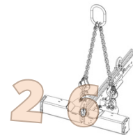
d&b audiotechnik CCL Flying Frame Set
